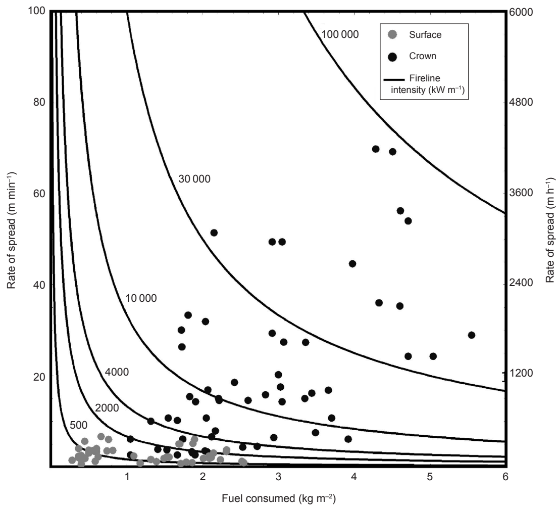
Figure 2. Head fire rate of spread and fuel consumed in relation to the type of fire and six distinct levels of Byram's (1959) fireline intensity (kW m -1 ), assuming a heat of combustion of 18 000 kJ kg -1 , for the experimental surface and crown fires used in the development of the fire spread functions included within the PPPY model system for predicting fire behaviour in pine plantations
